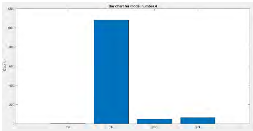
Figure 1. Bar Chart from x_2, x_1, x_7, x_{14}, x_4, x_6, x_3, x_{13}, x_8, x_{17}
